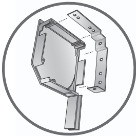
Reinforced bracket design for large patio installations
