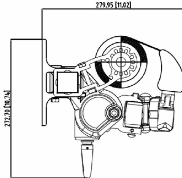
View with Wall Bracket and Aluminum Hood Elite Plus X-arm
