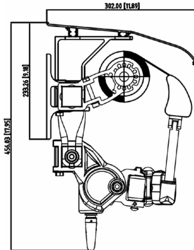
View with Wall Bracket and Aluminum Hood Elite Plus X-arm
